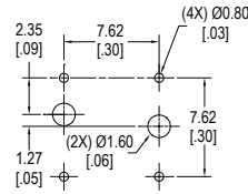
B Style, Standard LED
