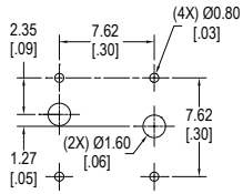
A Style, Standard LED
