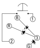
E Style, RGB LED
