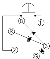
C Style, RGB LED
